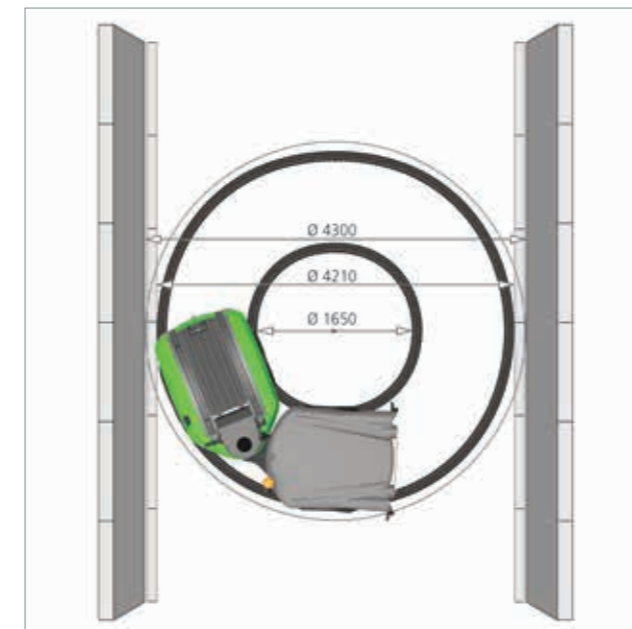
High manoeuvrability The City Ranger 3070 is articulated making it highly manoeuvrable in tight spaces. The inside turning circle of the basic machine is only 1650 mm.
